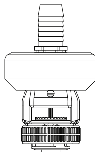
FOR D3000 AND A3000 SPRINKLERS ORIENT TAPERED END DOWN (NOT TO BE USED W/ THE RED D3000 CHEM. PLATE)
