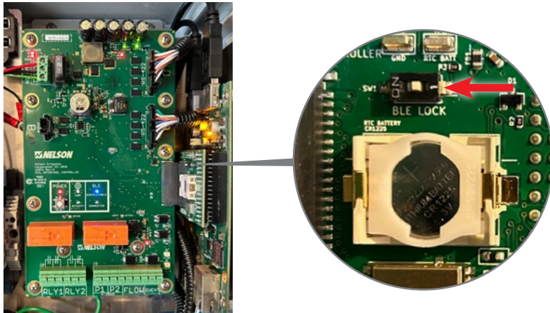
Fig. 1. The BLE Lock switch is located on the circuit board on the right side of the Twig-MC, just above the internal clock backup battery. When the switch is in the “ON” position, the Bluetooth® is locked and inactive.
